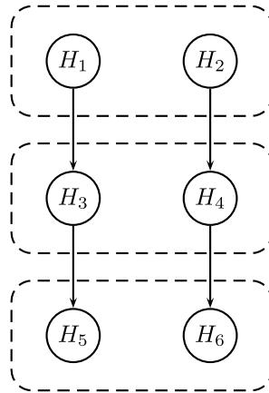
Figure 1 Ordering of the hypotheses in the clinical trial example. Families F_1, F_2, F_3 refer to the primary endpoint P, secondary endpoint S1, and secondary endpoint S2, respectively. Hypotheses H_1, H_3, H_5 refer to low dose versus placebo comparisons while hypotheses H_2, H_4, H_6 refer to high dose versus placebo comparisons.
